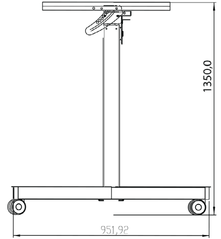
Top position / Table configuration: 1350 mm
