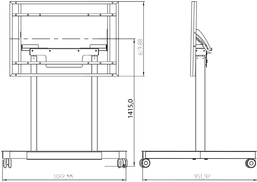
Top position / Trolley configuration: 1415 mm
