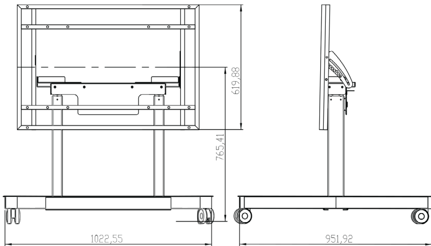
Bottom position / Trolley configuration: 765 mm
