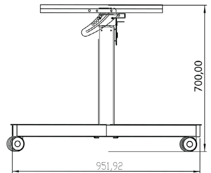
Bottom position / Table configuration: 700 mm
